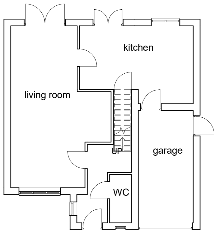
1 Ground floor 1 : 100
